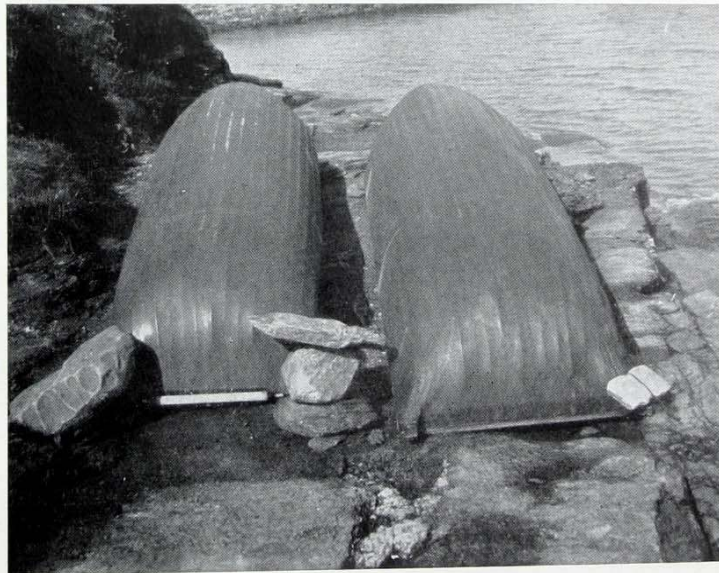
FIG. 2. TWO DUNFANAGHY CURRAGHS BOTTOM UP Photos by J. Hornell, 1936
