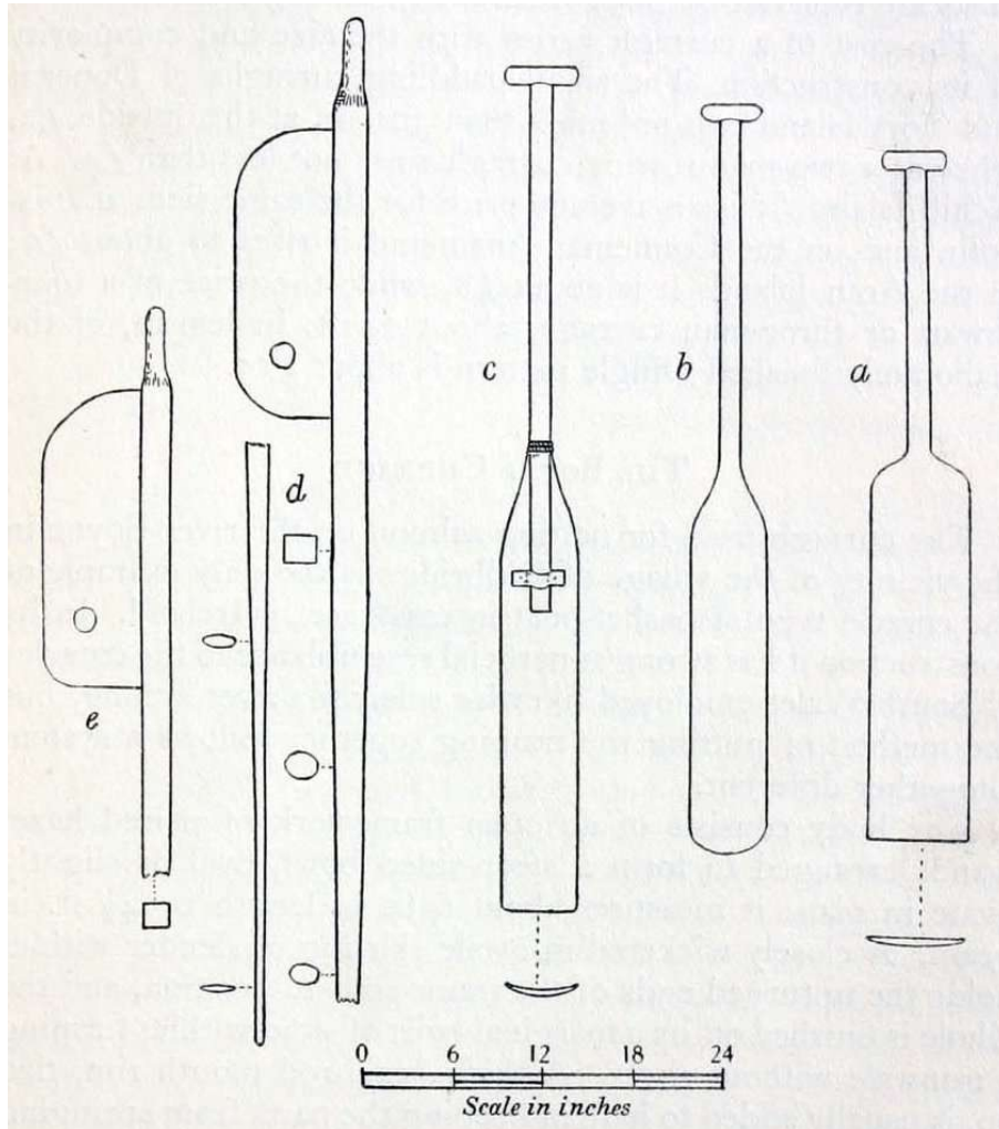
Text-fig. 1. Types of paddles and oars, a, paddle used on the Boyne; b, modern type of paddle, Donegal paddling curragh; c, old type of paddle, same locality; d, Sheephaven type of curragh oar; e, Mulroy Bay oar-local form of thole-pin block or "bull". (Original.)
