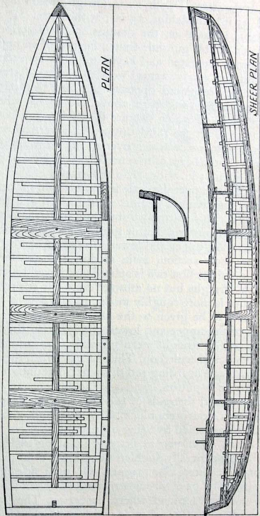
ACHILL ISLAND CURRAGH SCALE - 1 INCH TO 3 FEET 3 INCHES
