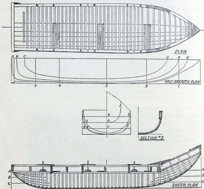
Plan 3.
