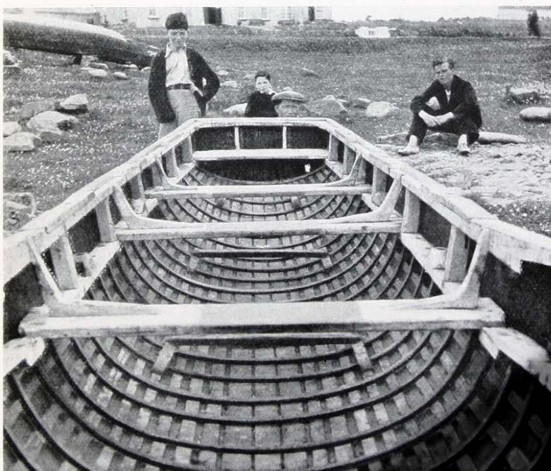
FIG. 2. LOOKING AFT INTO THE HULL OF A KILKEE CURRAGH Photos by J. Hornell, 1936
