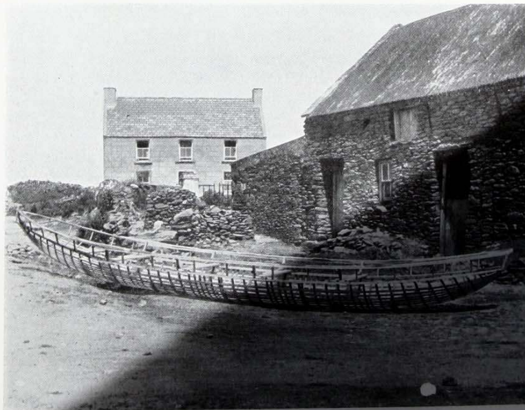
FIG. 2. SIDE VIEW OF THE FRAMEWORK OF A DINGLE CURRAGH
