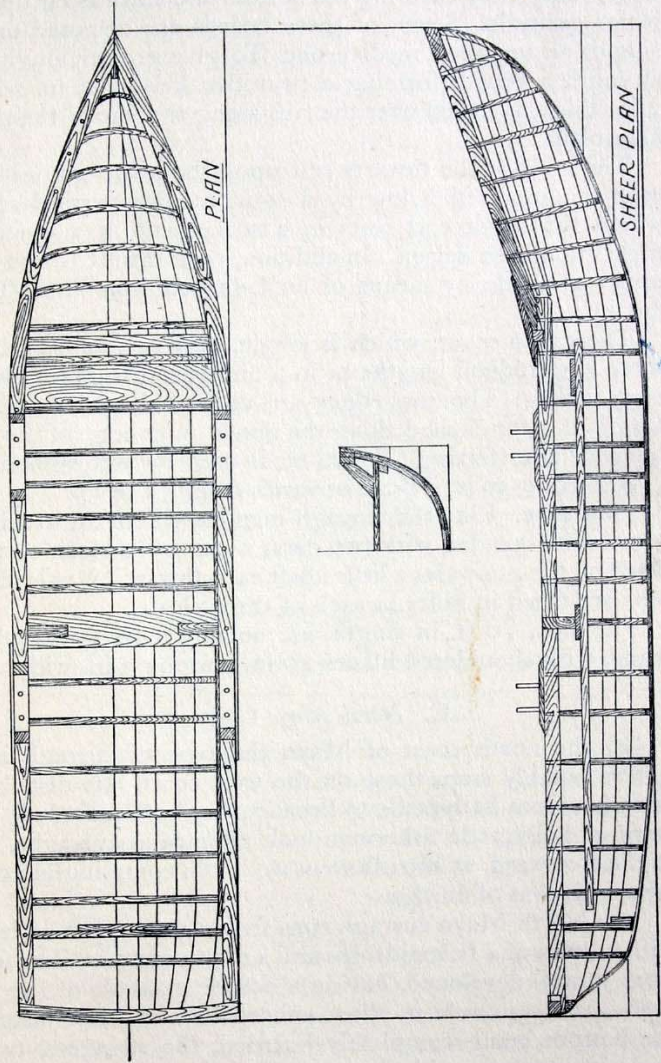
Plan 2.
