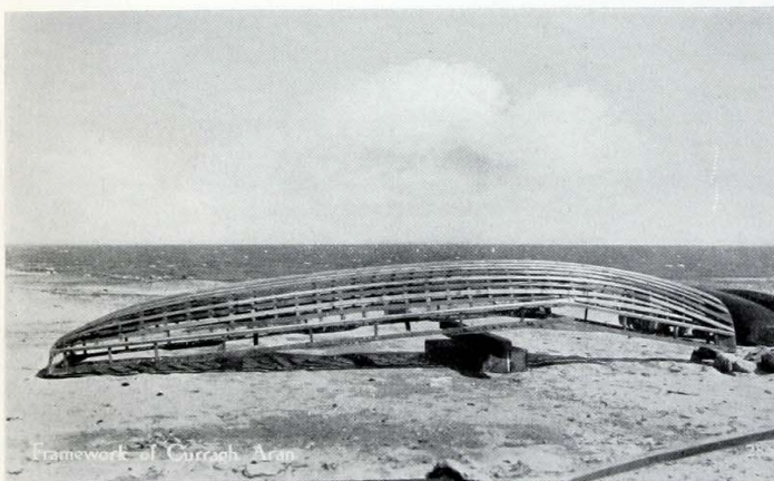
FIG. 2. A COMPLETED FRAMEWORK OF AN ARAN ISLANDS CURRAGH
