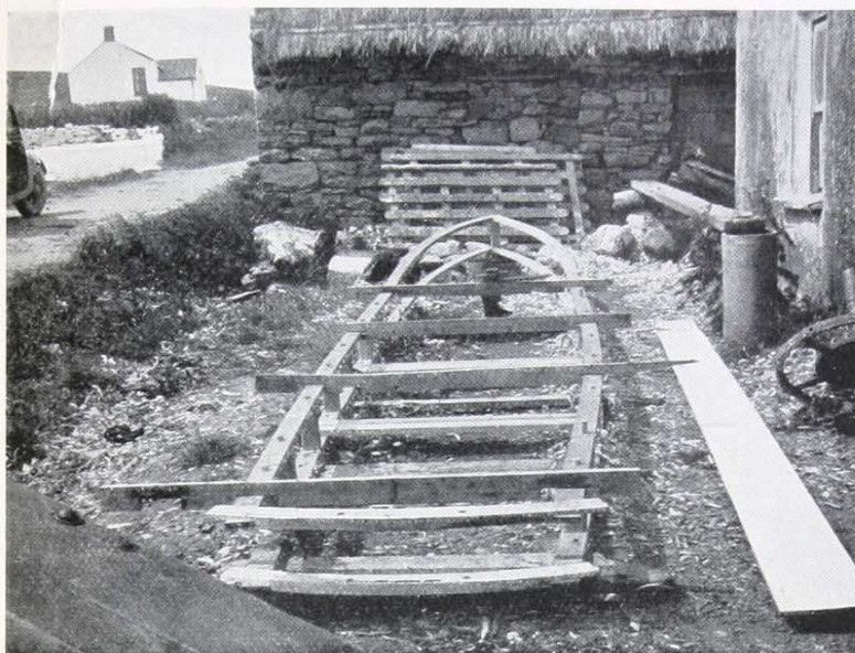
FIG. 1. BUILDING A KILKEE CURRAGH The gunwale frame has just been completed.
